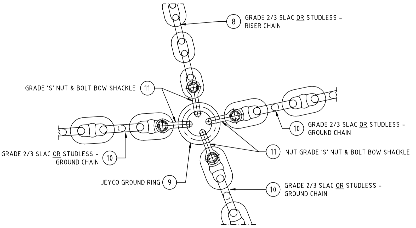
GROUND CONNECTION DETAILS
