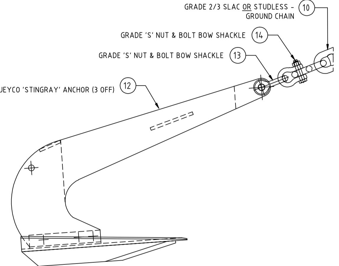
ANCHOR CONNECTION DETAIL
