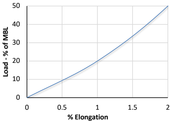
Jeyflex 12 Elongation (%)
