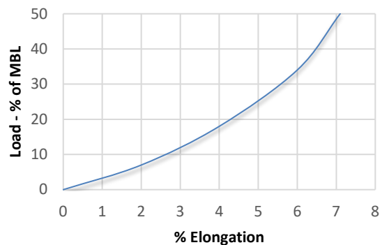
Polyester Double Braid Elongation (%)
