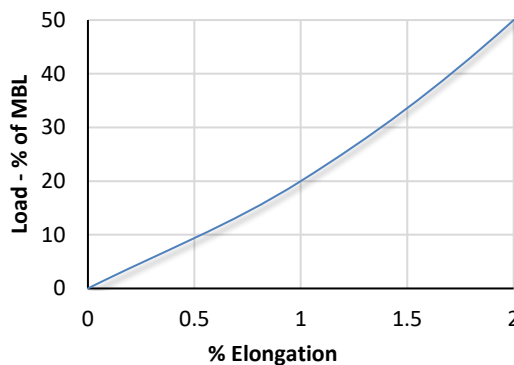
Texteel 12x12 Elongation (%)
