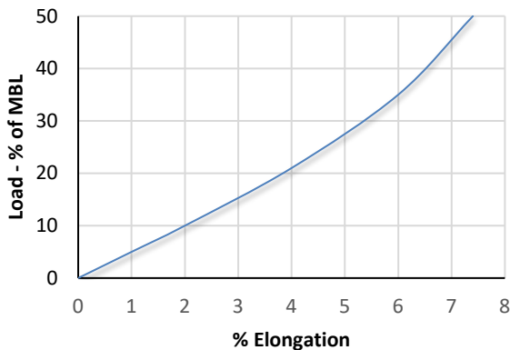
Towmaster Elongation (%)
